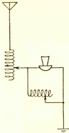
Fig. 4. Microphone With Shunted Inductance
