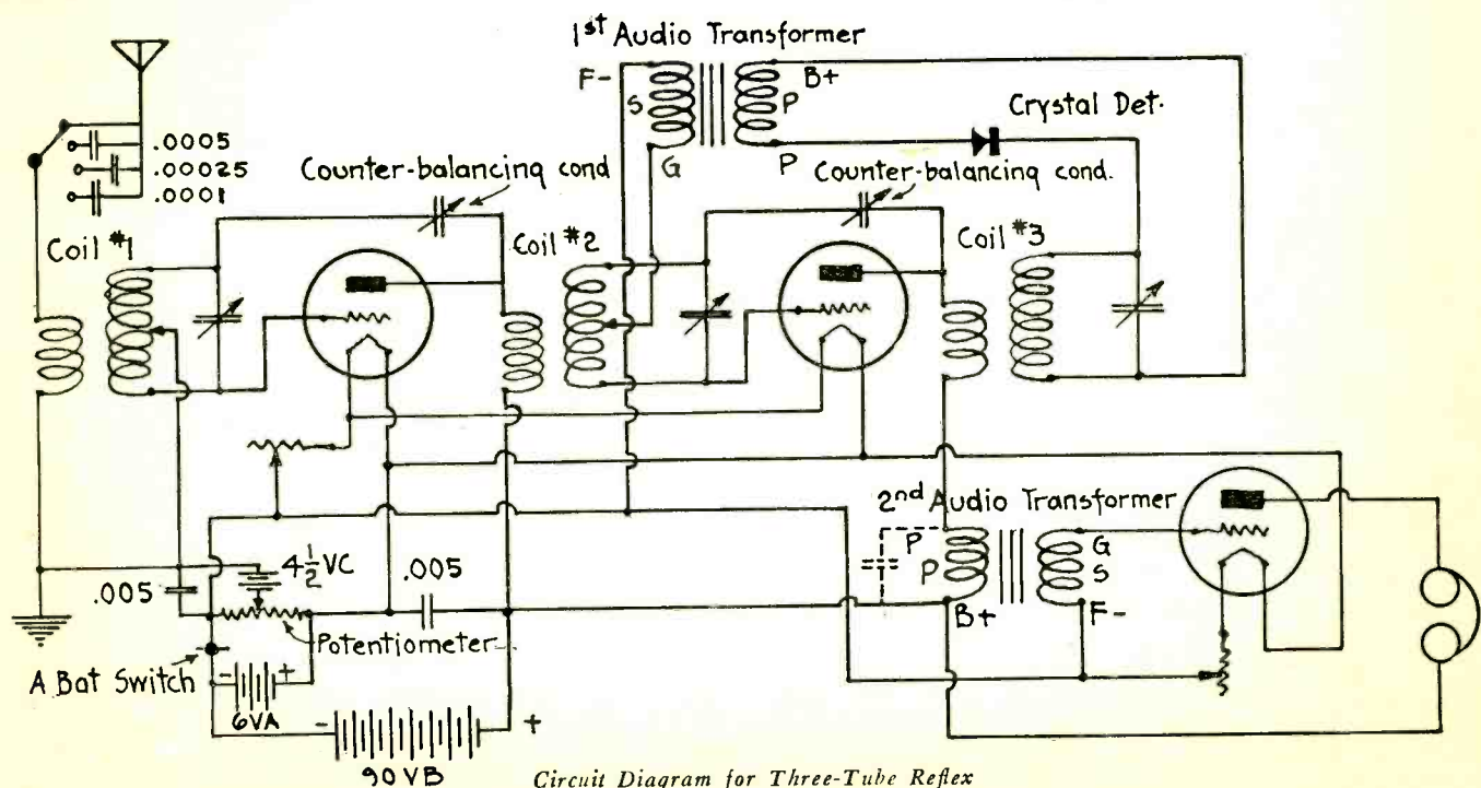
Circuit Diagram for Three-Tube Reflex
