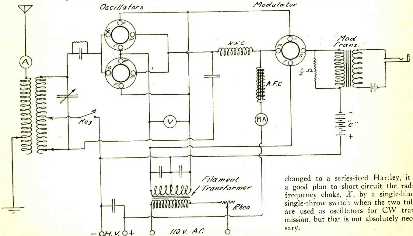
Fig. 6. Circuit Diagram of Shunt-Feed, Inductively-Coupled Hartley Transmitter with Heising Modulation
