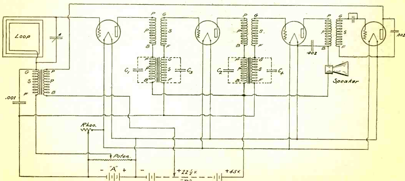
Circuit Diagram for Reflexed Triple R. F. and A. F. with Crystal Detector
