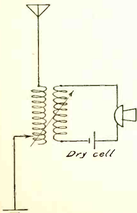
Fig. 3. Microphone in Coupled Circuit
