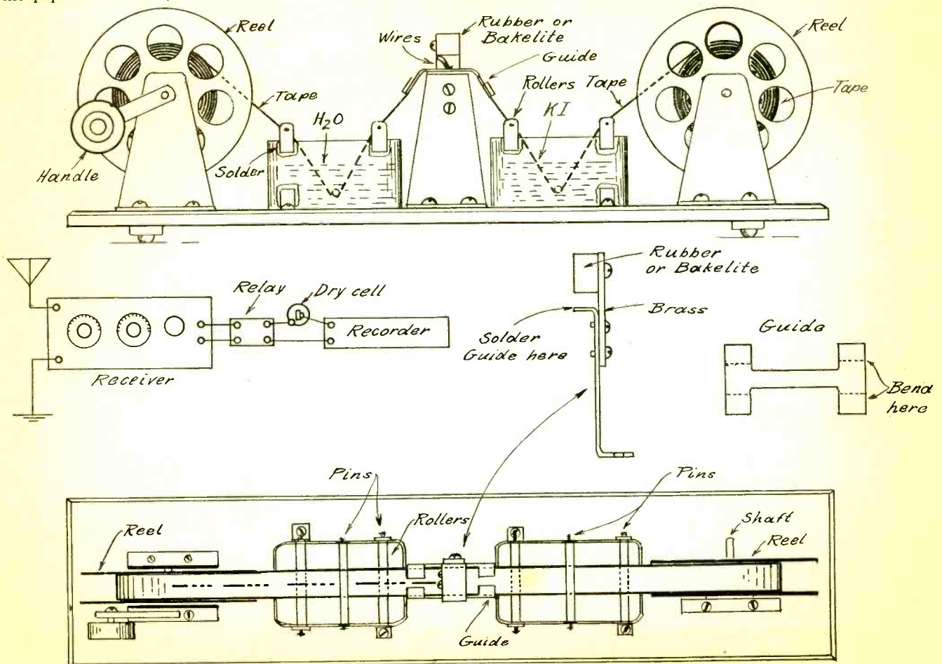
Constructional Details of Code Recorder
