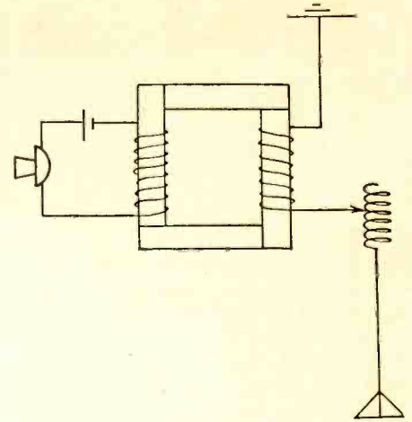
Fig. 5. Magnetic Modulator
