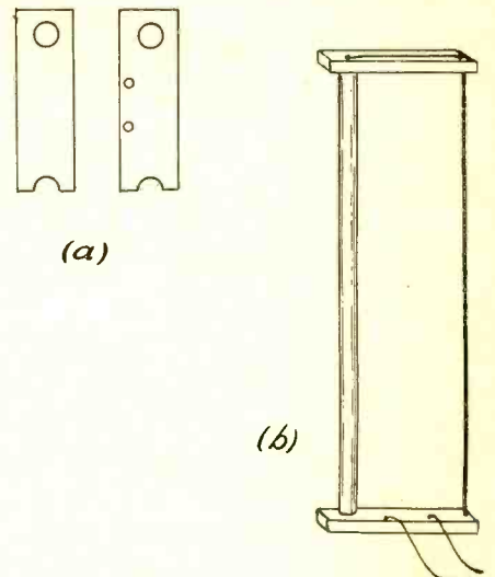
Fig. 4. Constructional Details of Single-Wire Loop
