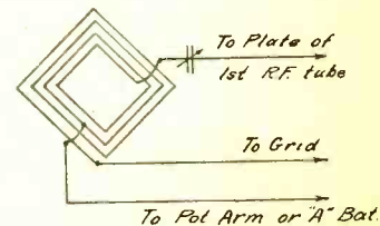
Fig. 5. Connection of Mid-Tap Loop
