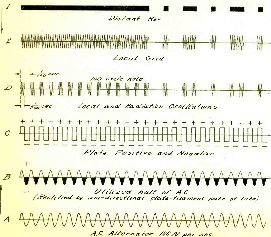
Fig. 3. Illustration of Tube Action
