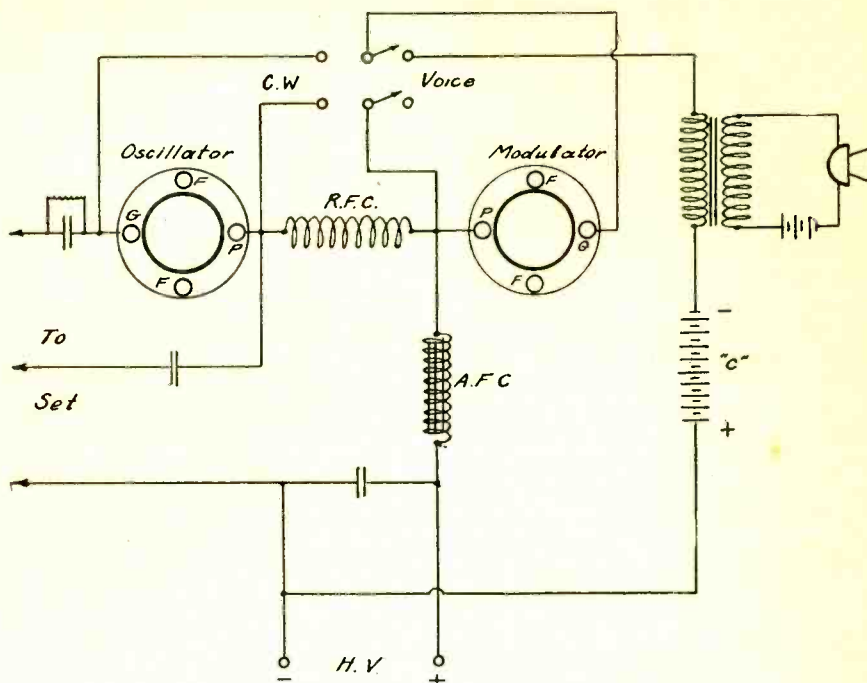
Fig. 4. Circuit Diagram with CW Phone Switch
