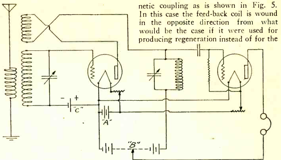
Fig. 5. Limitation of Regeneration with Reverse Feedback Coil.
