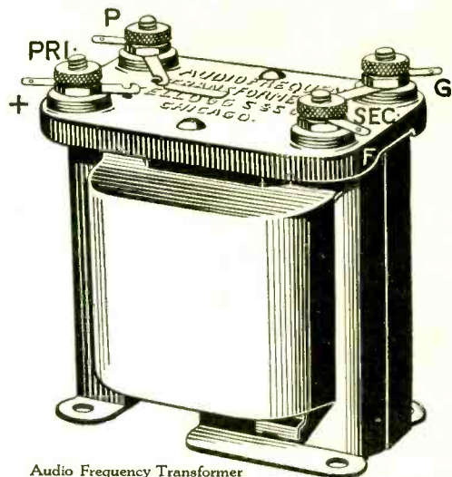
Audio Frequency Transformer
