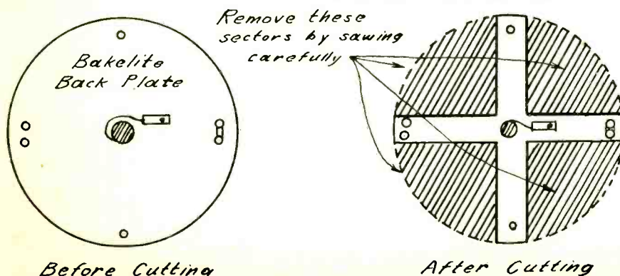
Fig. 2. Change in Condenser End Plates
