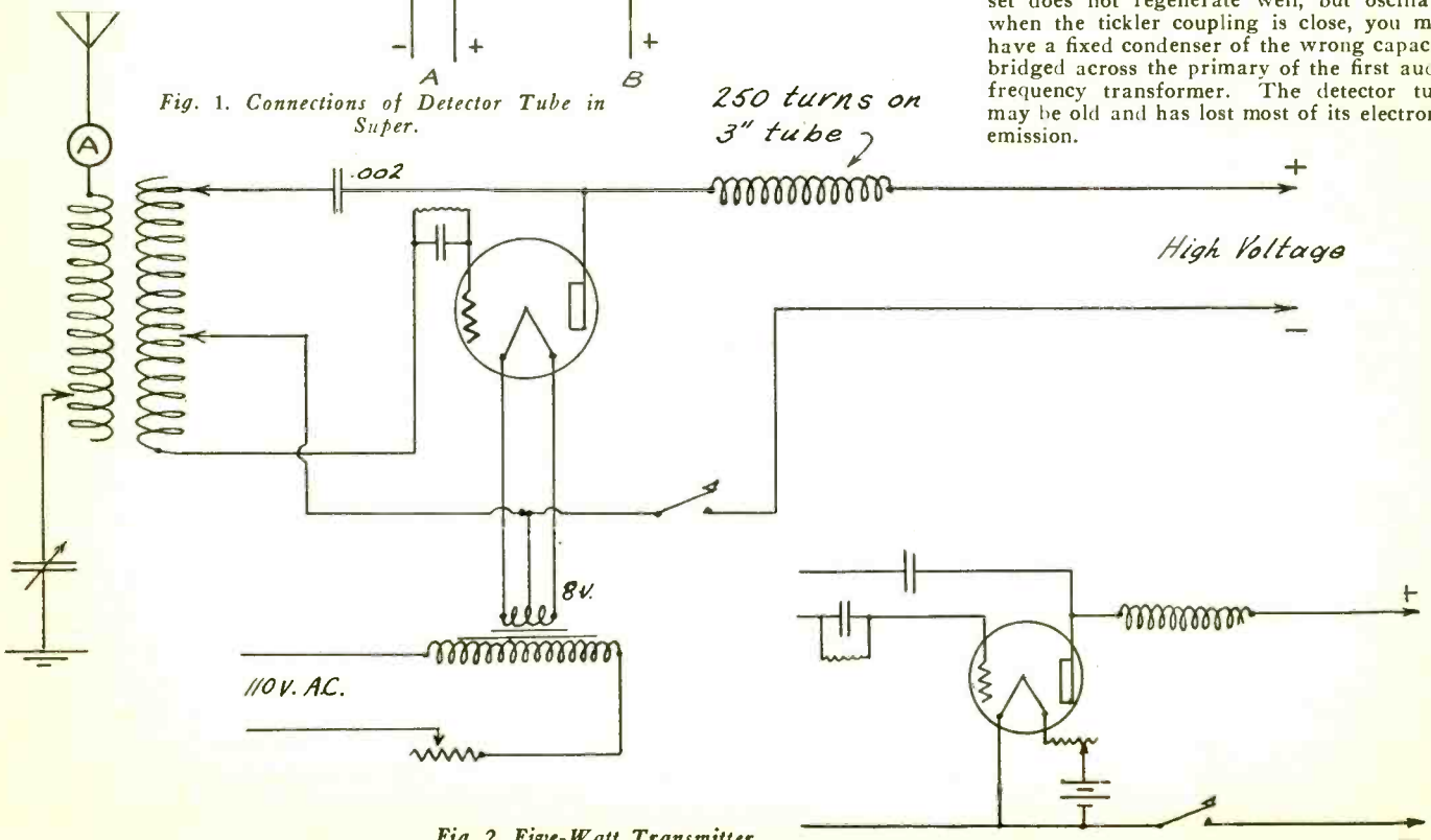
Fig. 2. Five-Watt Transmitter.
