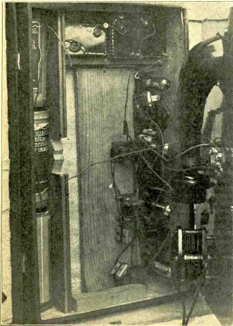
Inside View of Portable Receiver
