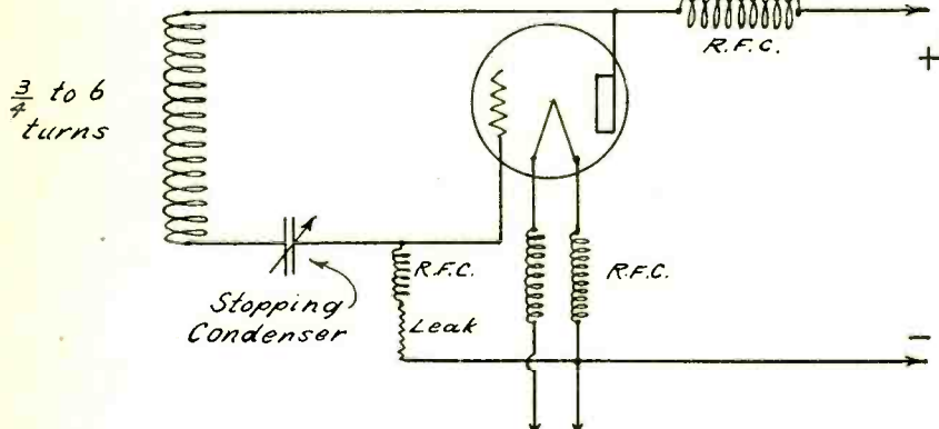
Fig. 1. Modified Colpitts Oscillator
