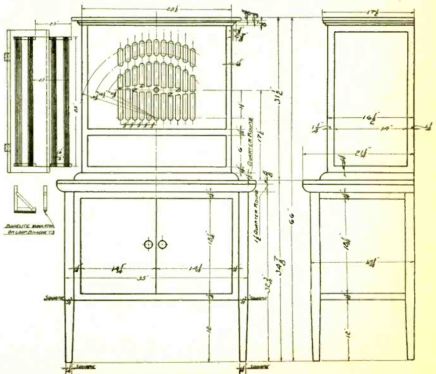
Constructional Details of Mr. Varney's Cabinet
