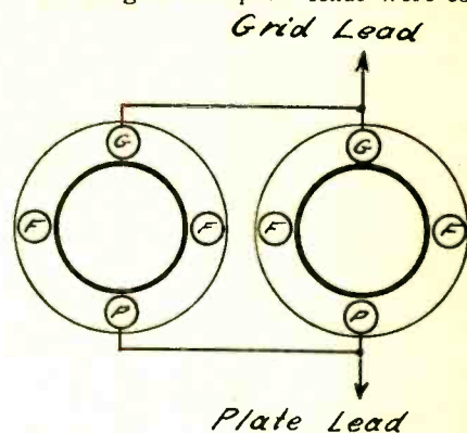
Fig. 3. Improper Method of Connection
