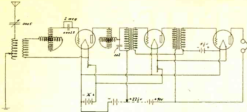
Fig. 3. Three-Circuit Regenerative Tuner with Variometer Control.
