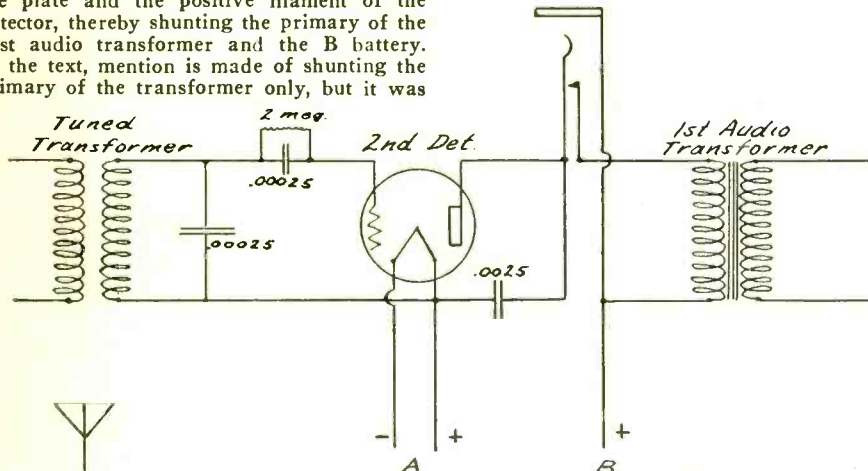
Fig. 1. Connections of Detector Tube in Super.
