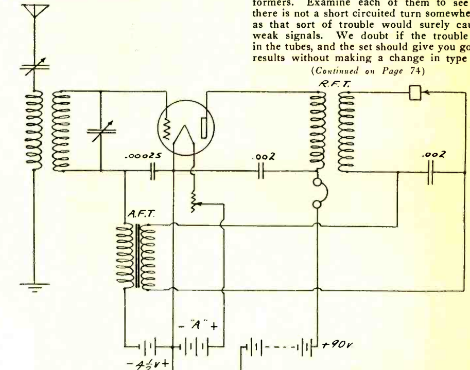
Fig. 5. Single Tube Reflex.
