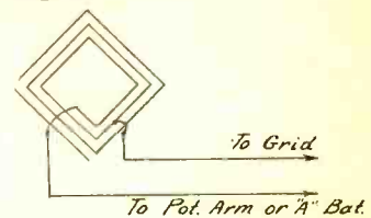
Fig. 4. Unused Turns of Short-Circuited Loop; Here Shown at Grid End, Should be at Filament End of Loop
