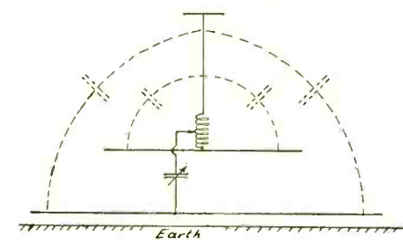
Fig. 4. Vertical Antenna with Counterpoise and Earth Shield
