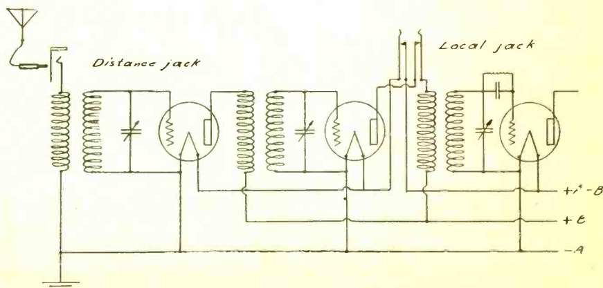
Modification of Neutrodyne to Give One Control
