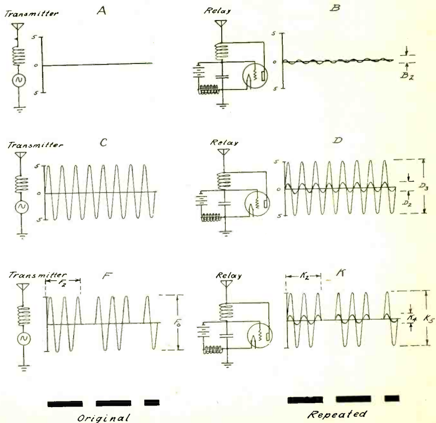
Fig. 2. Illustration of Relay Action
