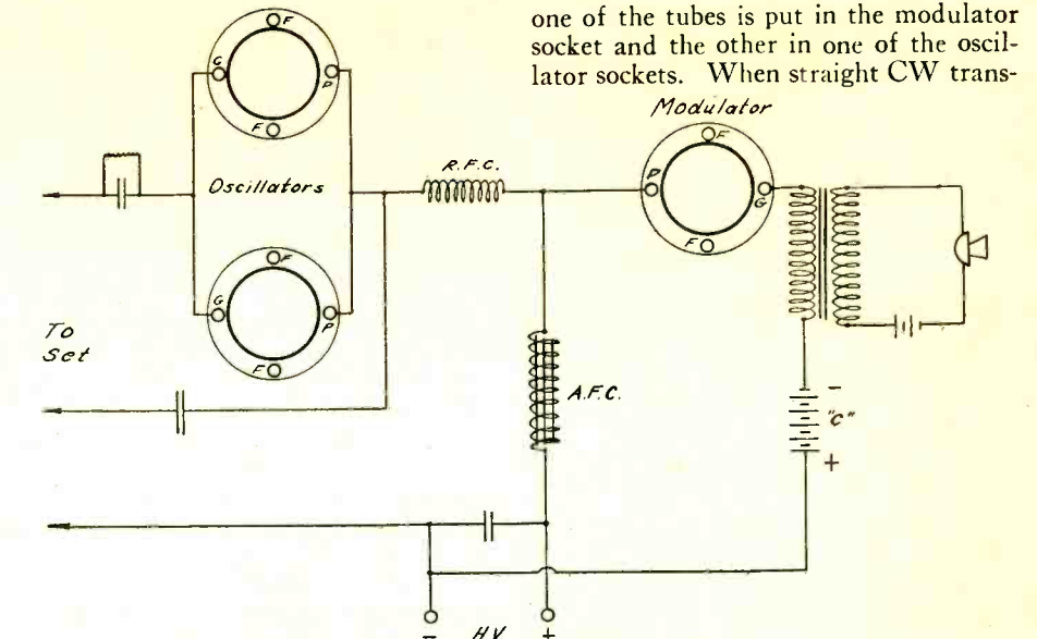
Fig. 5. Circuit Diagram Without Switch
