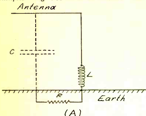
Fig. 1. Antenna and Ground With Equivalent Circuit
