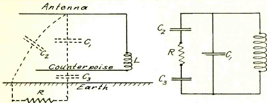
A Fig. 3. Antenna and Counterpoise With Equivalent Circuit B
