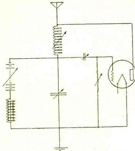
Fig. 1. Circuit Diagram for Tube Transmitter
