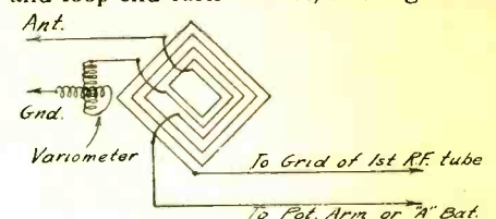
Fig. 2. Variometer Tuning of "Untuned Primary" on Loop
