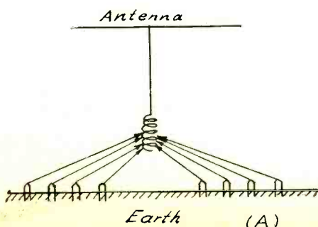
Fig. 2. Multi-Connection Ground
