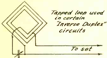
Fig. 6. Tapped Loop Used With Inverse Duplex Set
