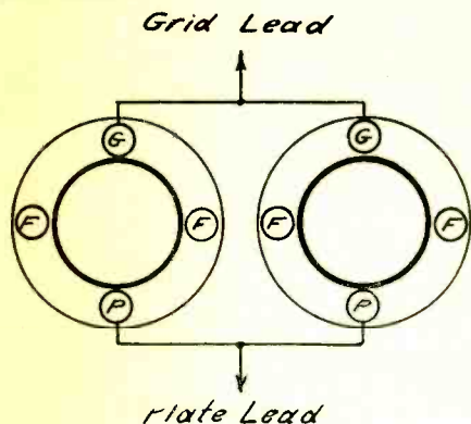
Fig. 1. Method of Connecting Two Sockets
