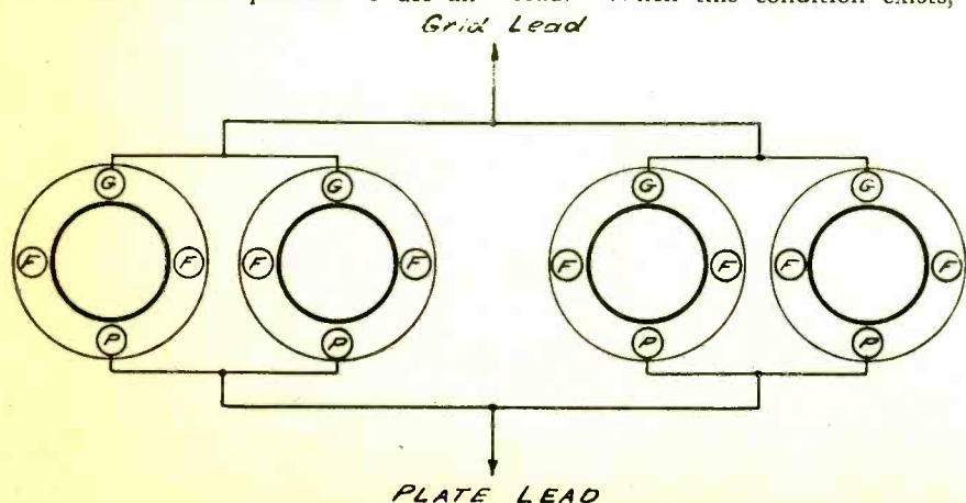
Fig. 2. Method of Connecting Four Sockets
