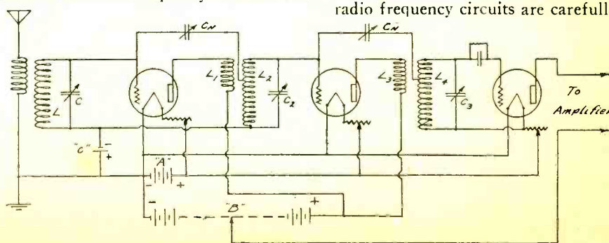
Fig. 2. Circuit Diagram of Neutrodyne Receiver
