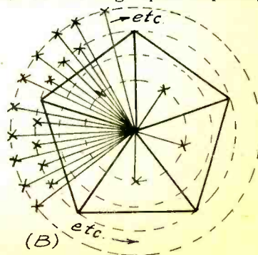
Fig. 2. Multi-Connection Ground
