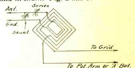
Fig. 3. Condenser Tuning of "Untuned Primary" on Loop
