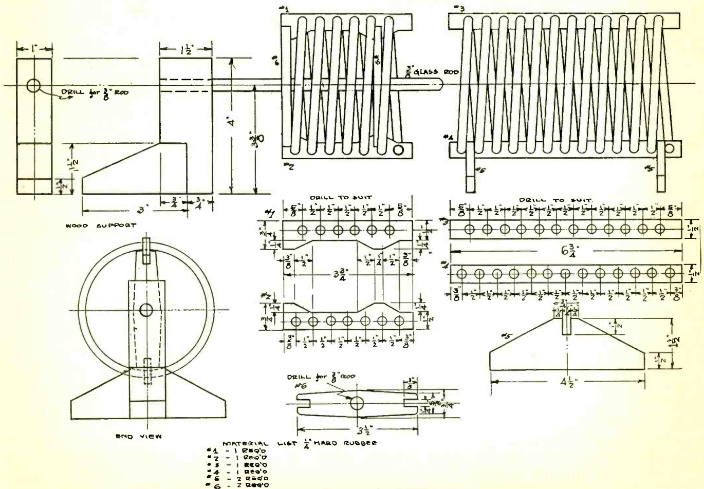
Constructional Details of Helix
