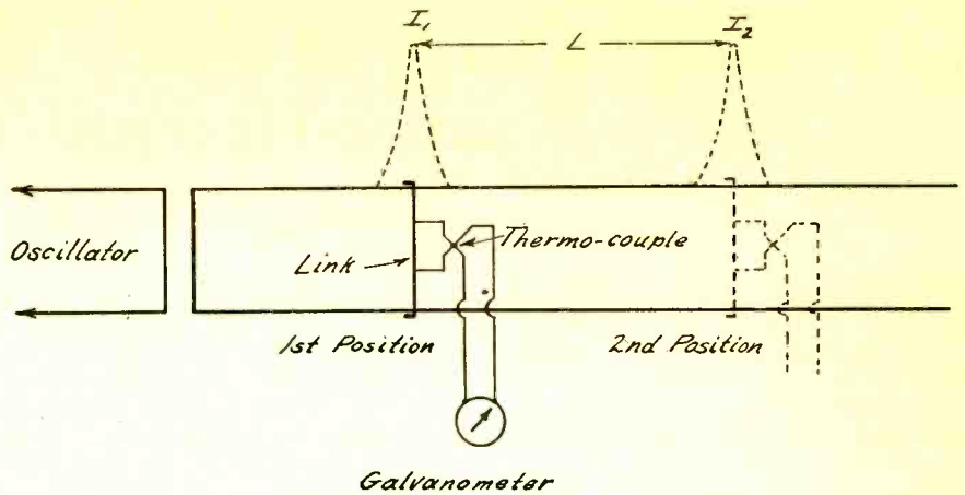
Fig. 2. Accurate Method of Measurement
