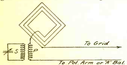
Fig. 7. Wave Trap with Loop set is tuned (with the trap condenser at
