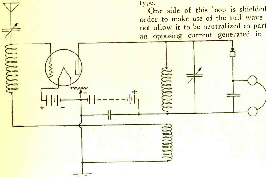
Fig. 1. Rounds No. 16 Circuit Diagram
